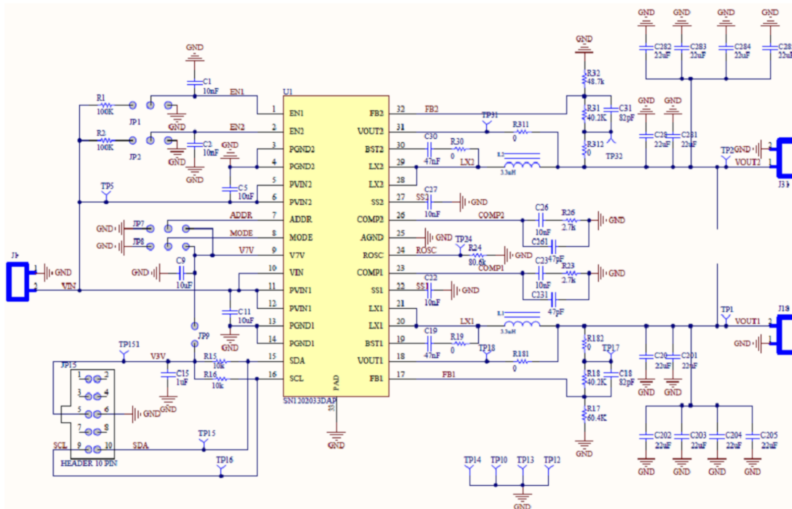
Figure 1. TPS65276V Schematic
